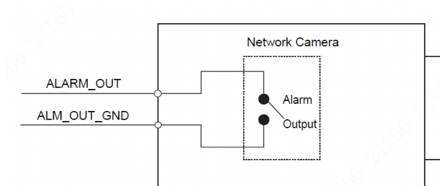
Figure 1-3 Alarm output
