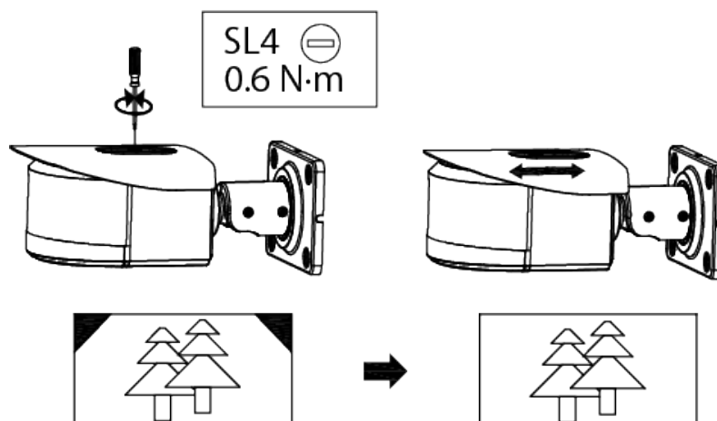
Figure 3-7 Adjust sunshield
